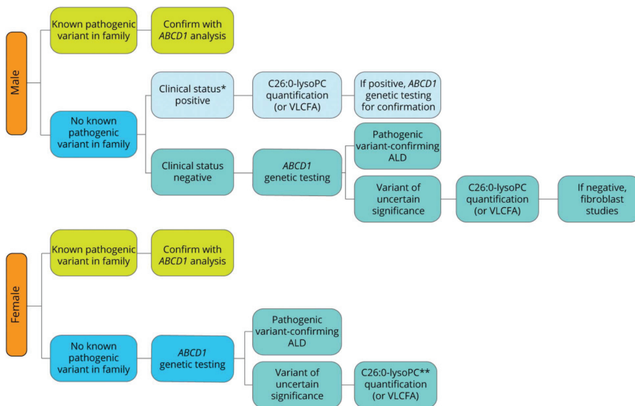
Figure 3 Diagnostic Algorithm
